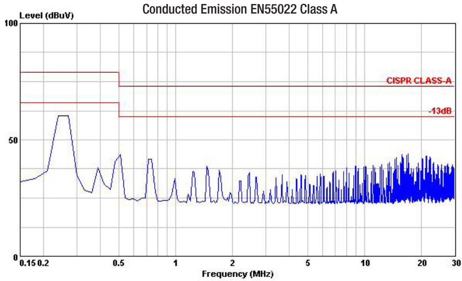
RP240H-2405SRW
