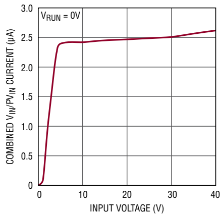
Shutdown Current on V IN /PV IN vs Input Voltage
