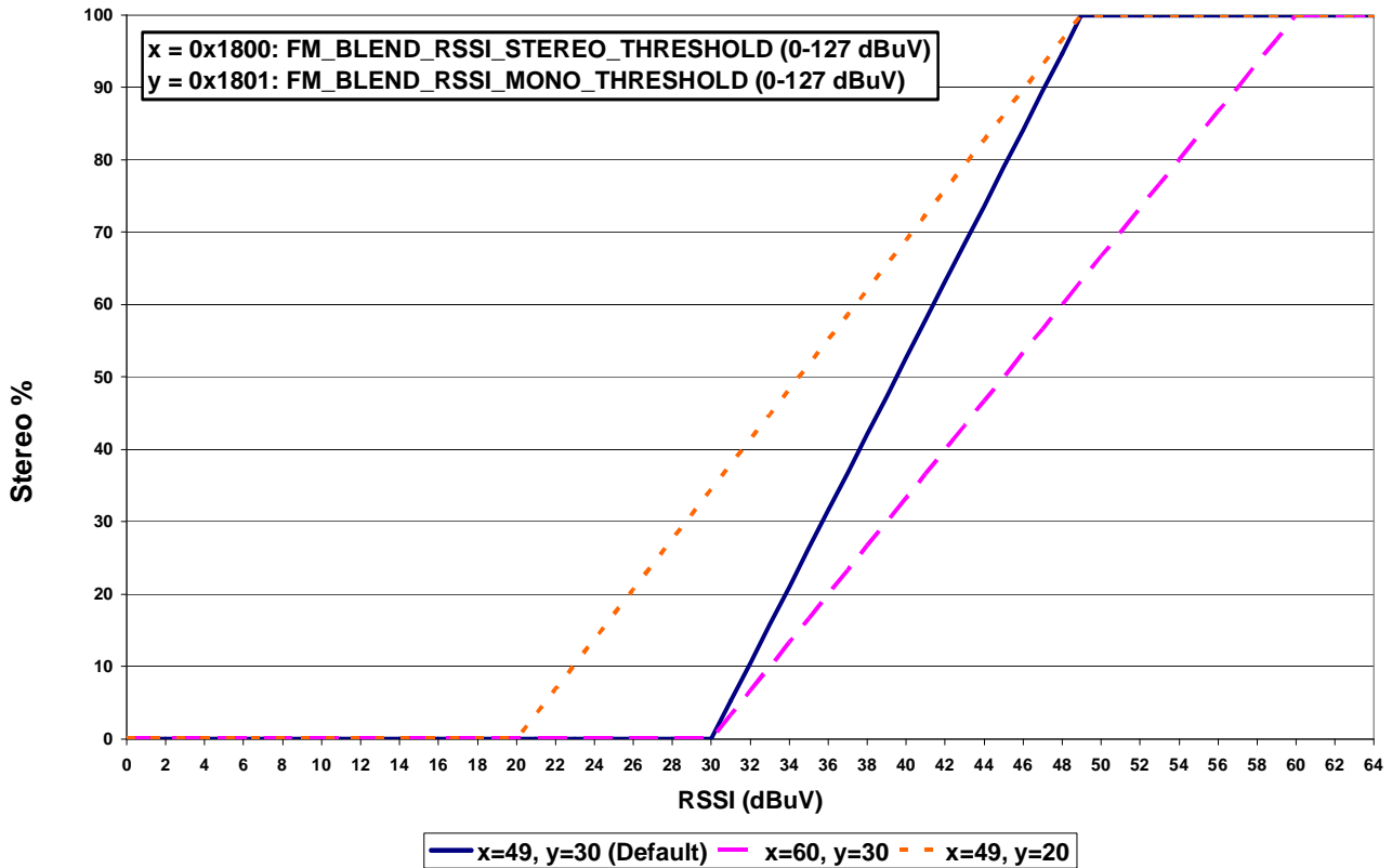
Figure 4. RSSI Blend
