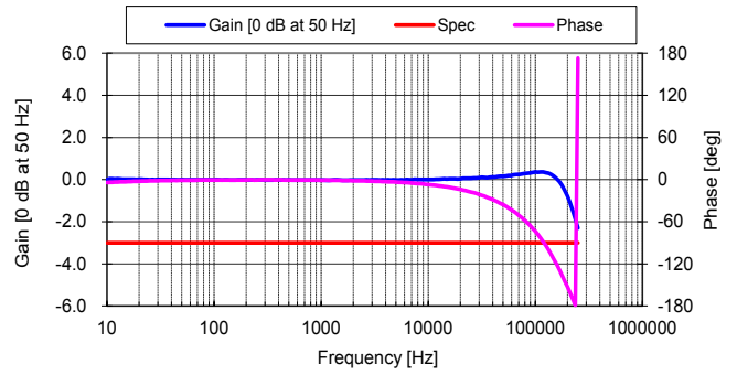
Figure 12: Frequency response
