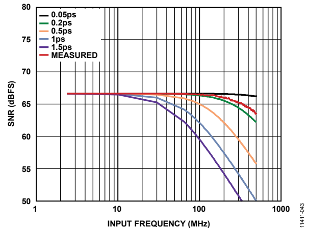
Figure 43. SNR vs. Input Frequency and Jitter
