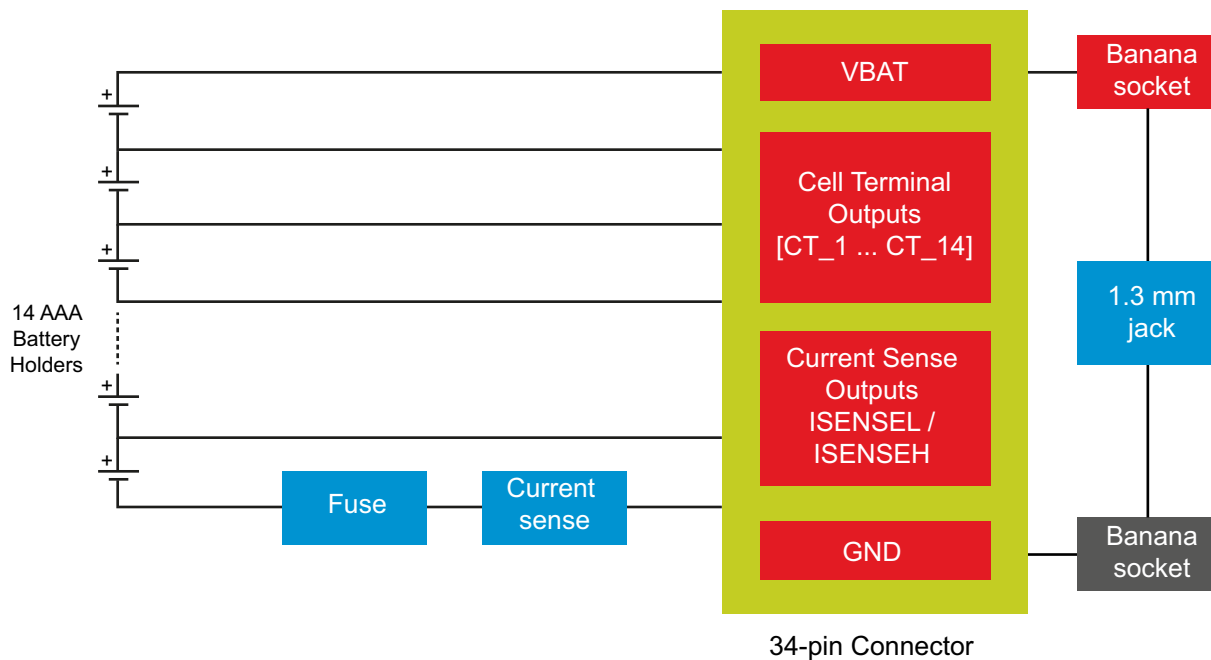
Figure 2. BATT-14AAAPACK Block Diagram
